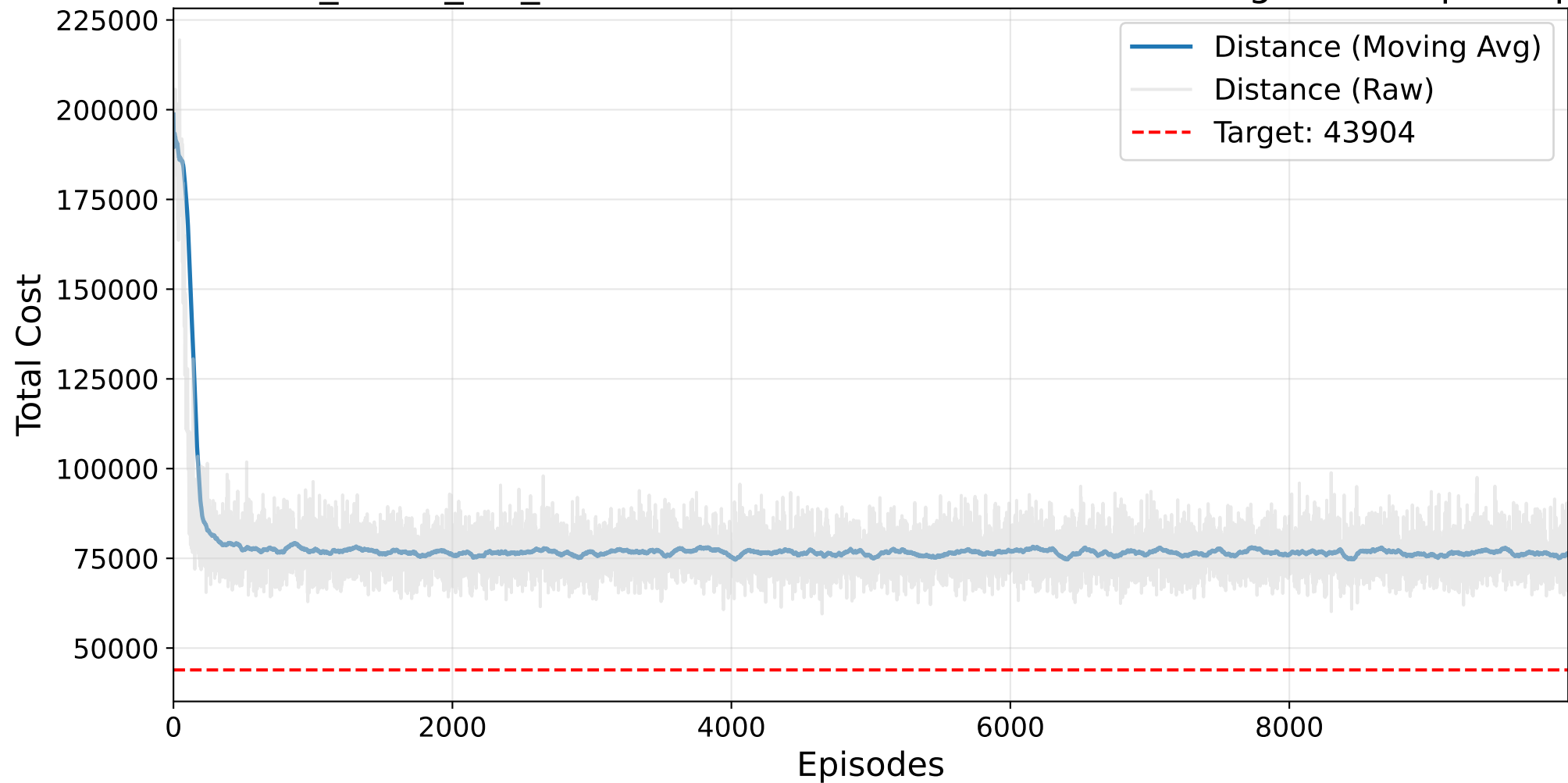
Final NO_MASK_NO_BAYESIAN Masked AutoRL-SOP Training - kro124p.3.sop
